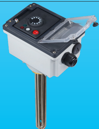
Y7 Measurement on rear mounted immersion heater (We do not supply the immersion heater)
