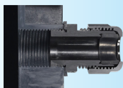
With usual M20 cable gland
